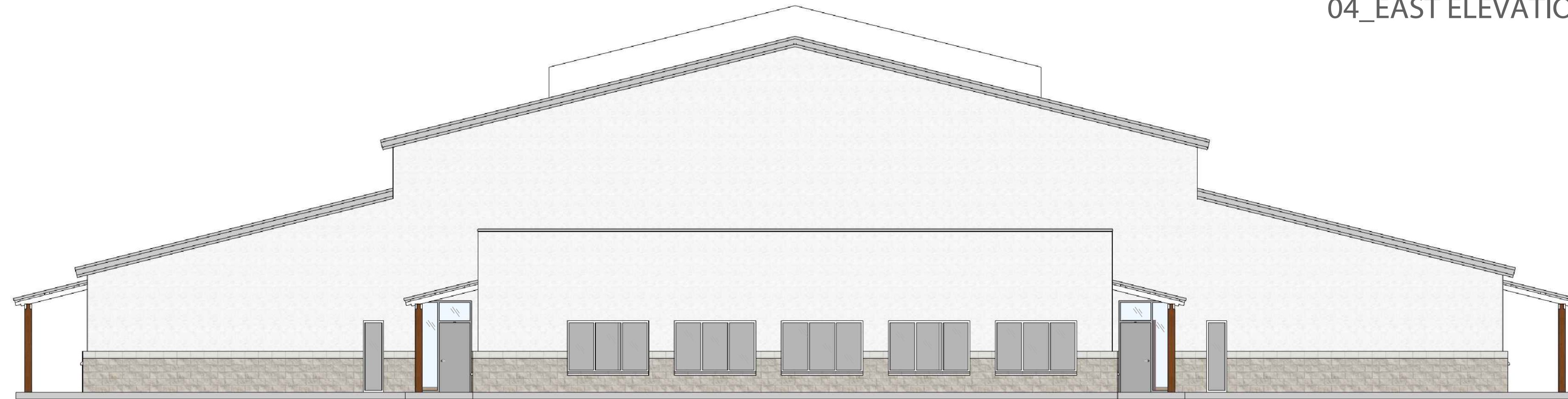
03_SOUTH ELEVATION
